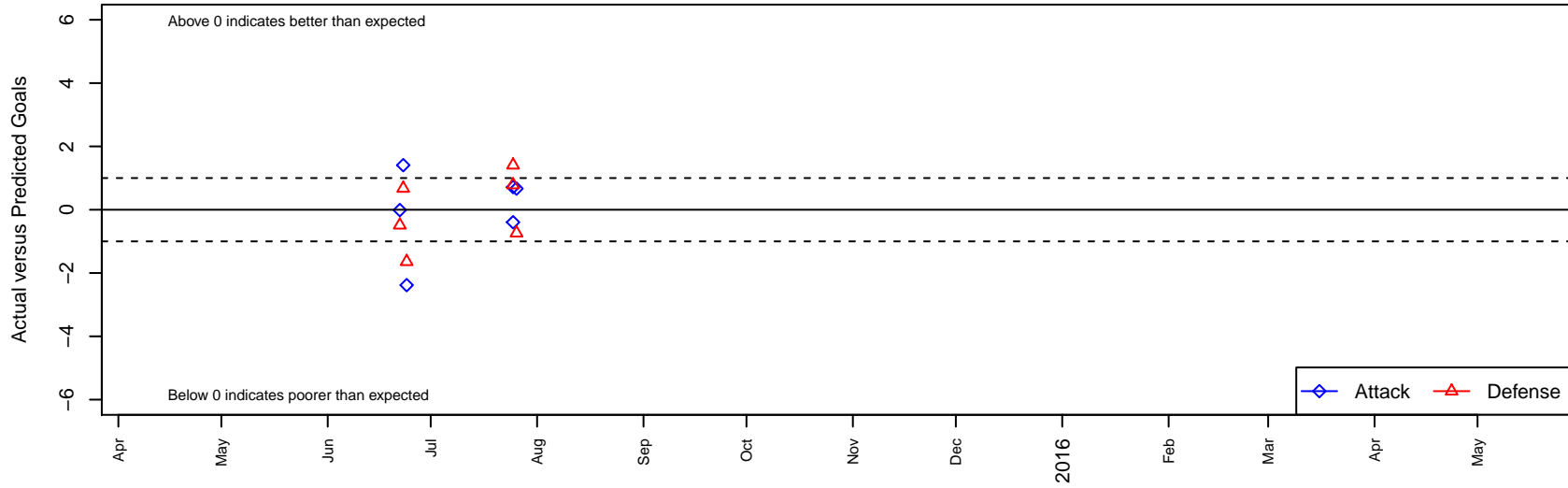
Broomfield Blast 01 Red G00 Dots are actual minus expected GF (blue circles) and GA (red triangles). Blue line is smoothed change in attack strength. Red is smoothed change in defense strength.
